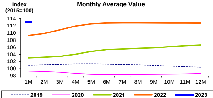
TH: Construction Materials Price Index: Monthly Average Value (Iron and Steel Products)
